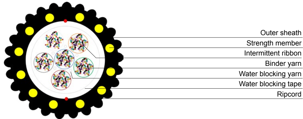
Typical structure 2: Duct pull type
