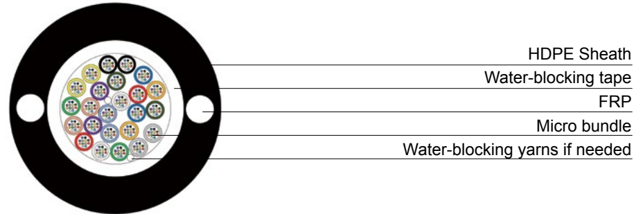
Drawing of duct cable up to 288Fo (Modularity 12)
