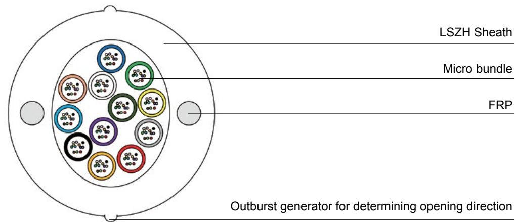
Drawing of riser cable 12 to 288Fo (Modularity 12)
