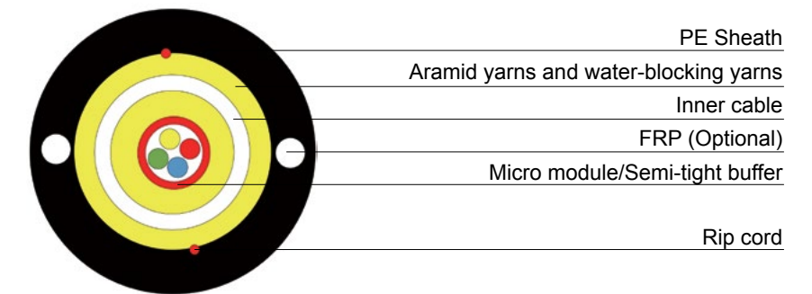
Drawing of outdoor and indoor drop cable 1 to 4Fo
