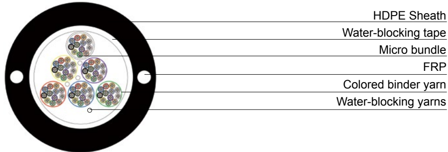
Drawing of duct cable 432 to 864Fo (Modularity 12)
