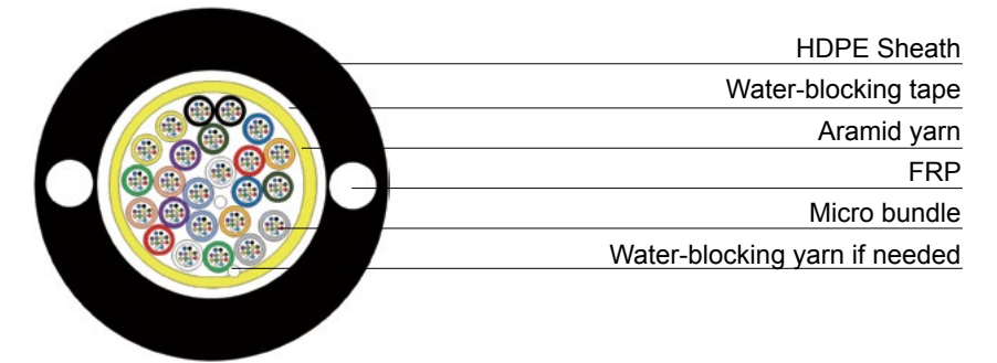
Drawing of aerial cable 12 to 288Fo (Modularity 12)
